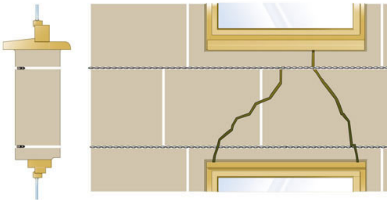
Repair of Failed Lintels in stone walls using Thor Heliforce bars
