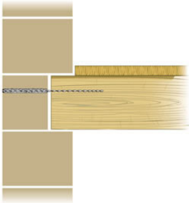
Restraining a bowed stone wall using Thor Drive Fix Restraint Ties into Joist end
